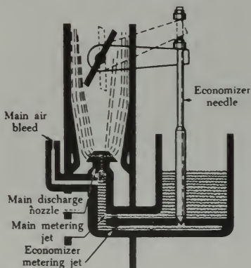
FIGURE 3-14. A needle-valve type economizer system.
